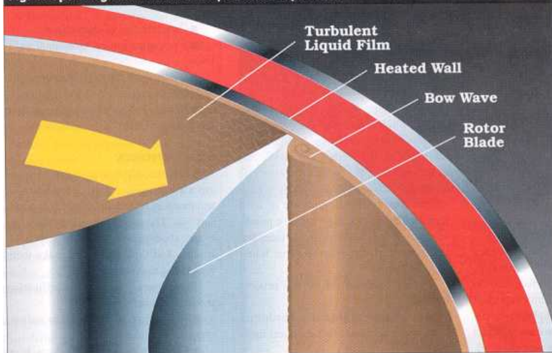
Fig. 1. Operating mechanisms of wiped-film evaporation.
