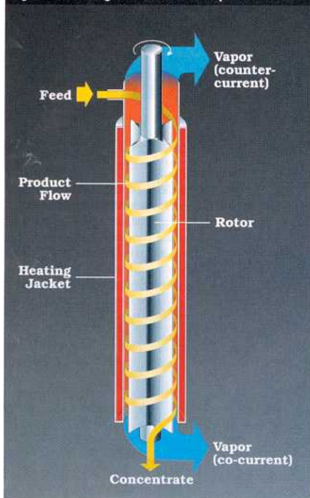
Fig. 2. Vertical agitated thin-film evaporation.
